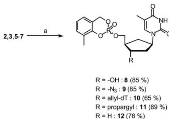
Scheme 3. (a) 3-methyl-cyclosaligenylphosphorochloridate, pyridine, -40 °C, 2 h.
