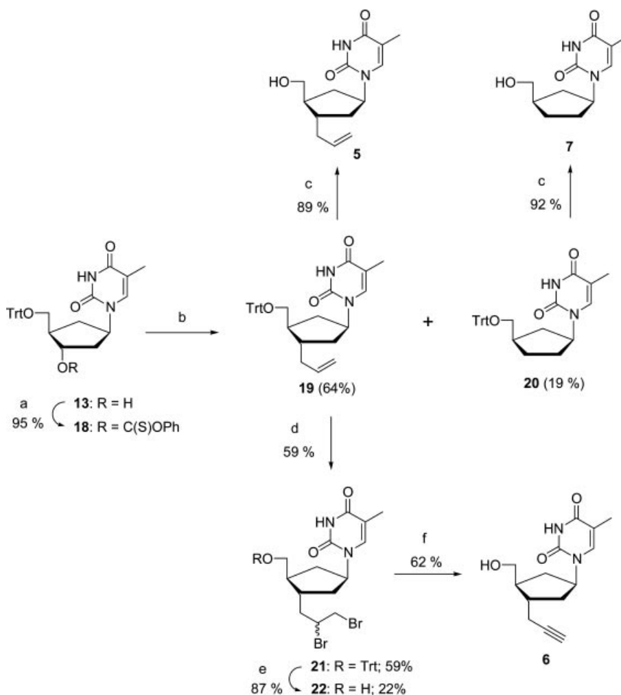
Scheme 2. (a) PTC-Cl, pyridine, CH 2 Cl 2 , room temp., 12 h (b) n Bu 3 Sn-allyl, AIBN, toluene, 80 °C, 48 h (c) TFA, CH 2 Cl 2 /MeOH, room temp., 12 h, (d) Br 2 , CCl 4 , -10 °C, 1 h (e) TFA, CH 2 Cl 2 /MeOH, room temp., 12 h (f) KOH, EtOH/H 2 O, reflux, 20 h.
