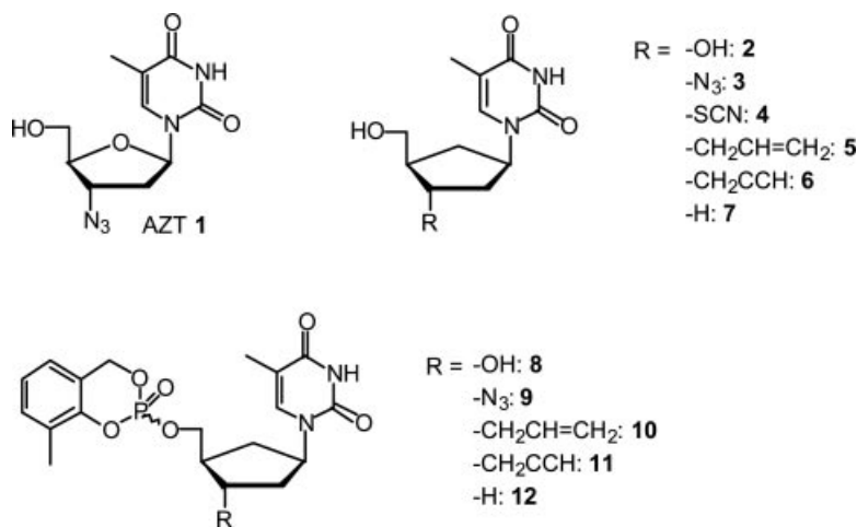
Figure 1. Carbocyclic nucleoside analogues and their corresponding cycloSal -phosphates.
